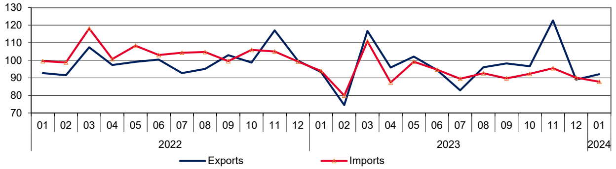
Figure 3. Volume index 2022–2024 2020 = 100
